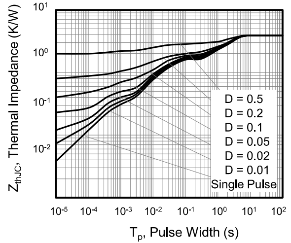
Figure 11. Transient Thermal Impedance TO-220F
